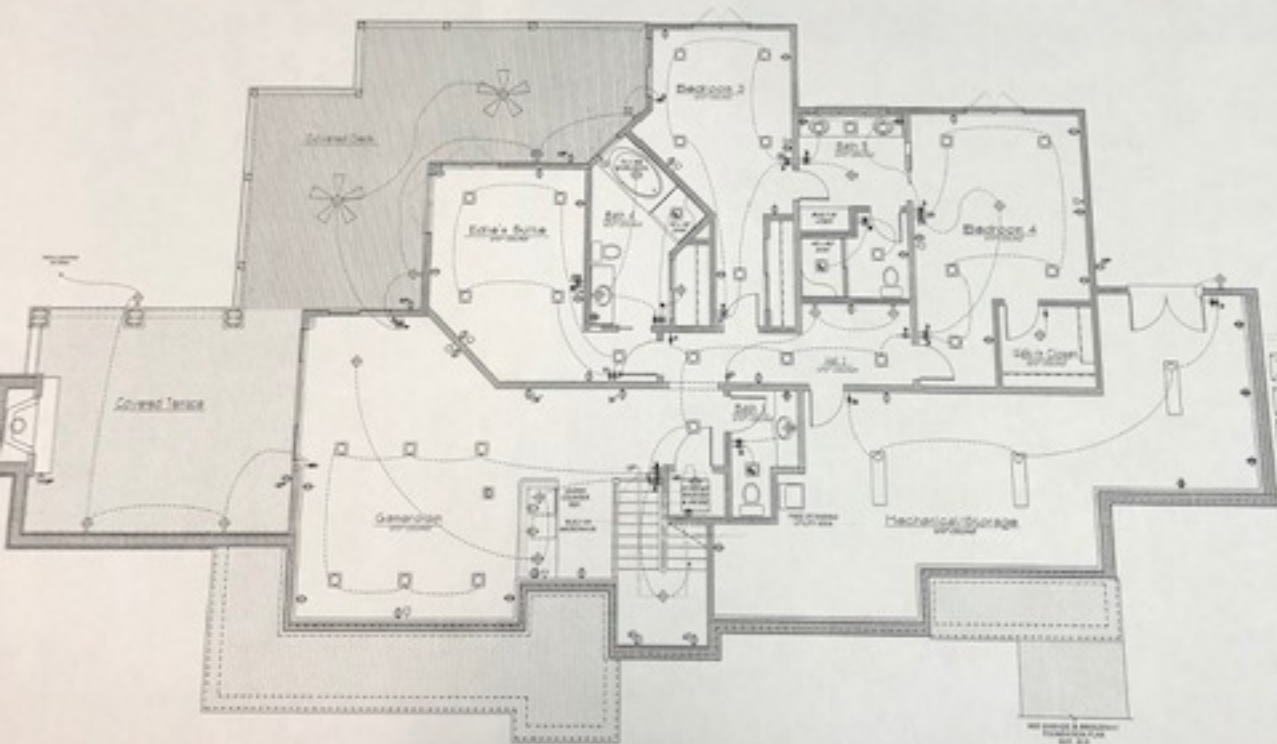
Lower Level Plan SCALE 1/4"=1'-0"
