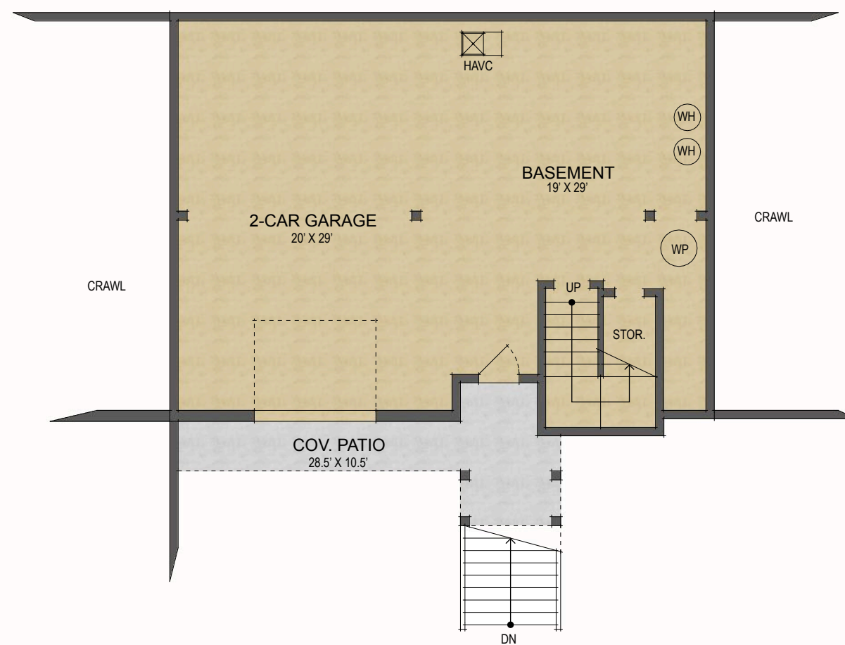
Lower Level Floor Plan
