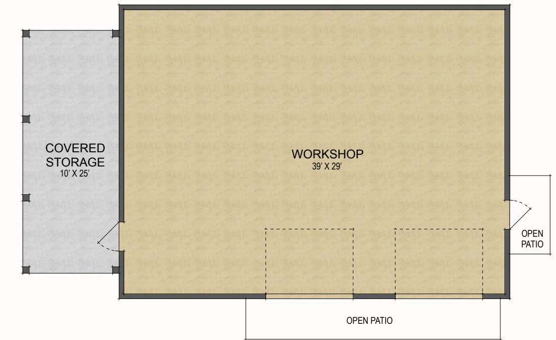
Workshop Floor Plan
