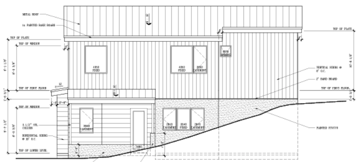
LEFT SIDE ELEVATION SCALE 1/4" = 1'-0"
