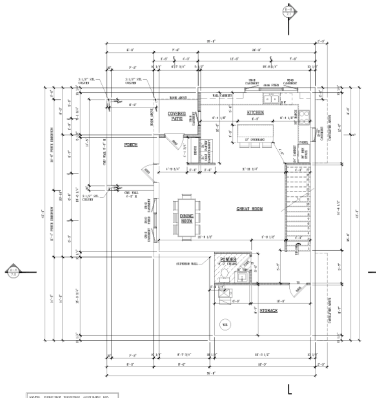
LOWER LEVEL PLAN SCALE 1/4" = 1'-0"
