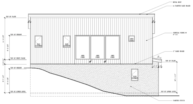
RIGHT SIDE ELEVATION SCALE 1/4" = 1'-0"
