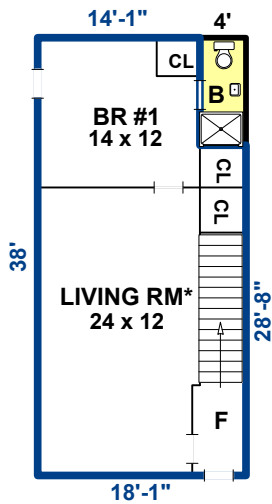
FIRST LEVEL 650 SF
