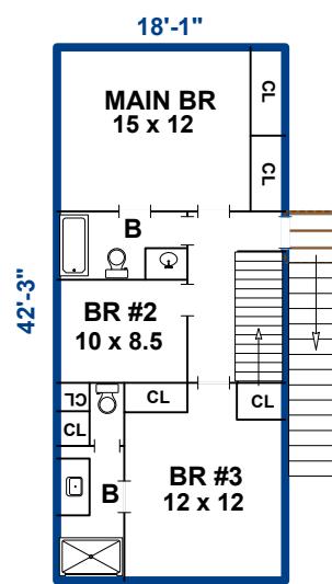
THIRD LEVEL 764 SF
