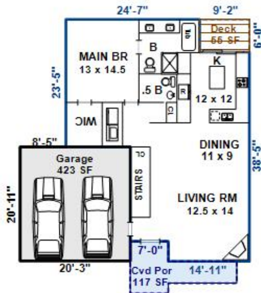
MAIN LEVEL 1170 SF
