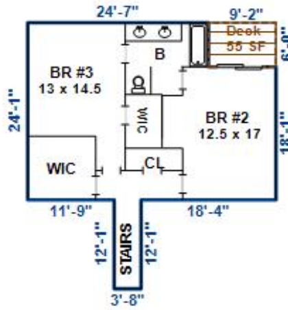
SECOND LEVEL 802 SF
