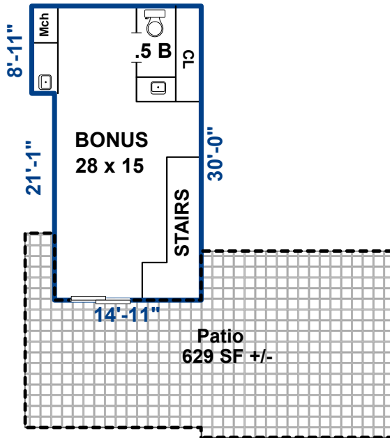
THIRD LEVEL 468 SF 17'-3"
