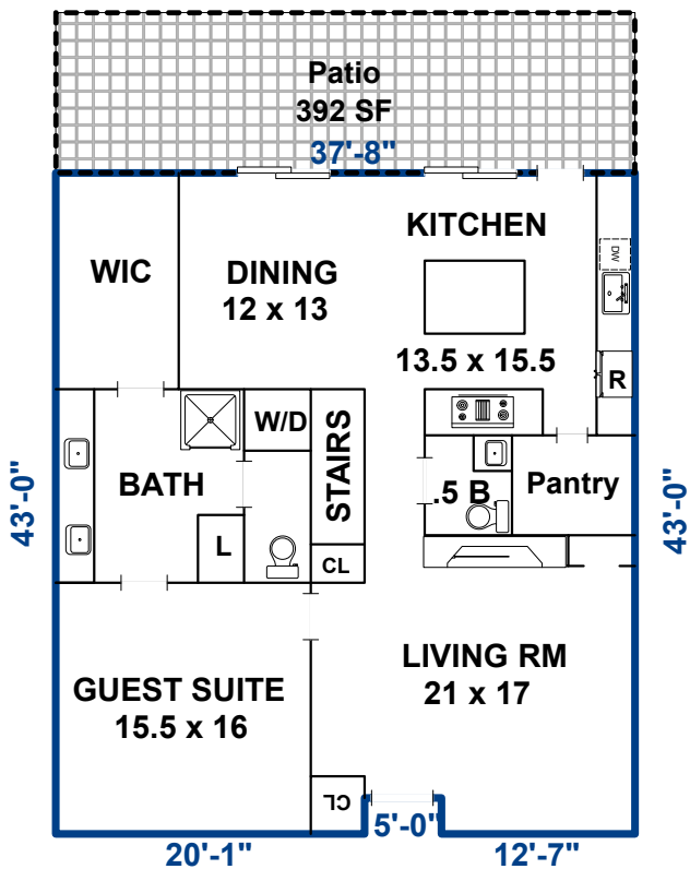
MAIN LEVEL 1608 SF
